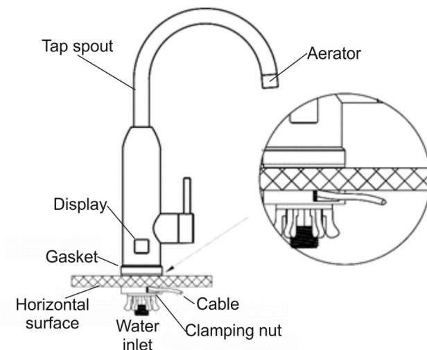
Fig. 2. Installation with the output of the power cable under the sink
