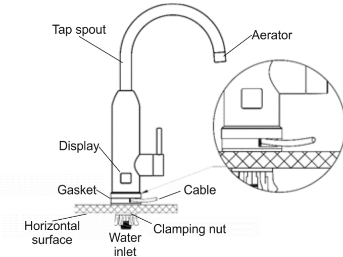
Fig. 1. Installation with the output of the power cable above the sink
