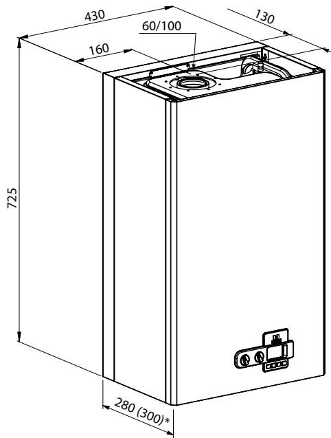
THERM 18 KD, KDZ, KDC; 25 KD, KDZ, KDC * THERM 35 KD, KDZ
